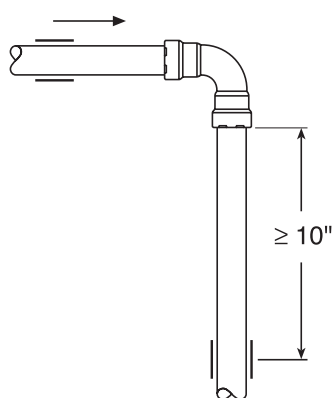
Figure 3.9 Spacing for sliding pipe hanger
