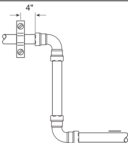
Figure 3.8 Spacing for sliding pipe hanger
