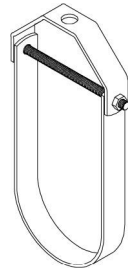
FIG. 430 INSULATED PIPE CLEVIS PAGE 49
