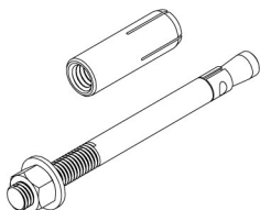
FIG. 47 CONCRETE ANCHORS PAGE 26
