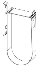
FIG. TRH 2 - TRH 5 TRH HANGING SYSTEM PAGE 39
