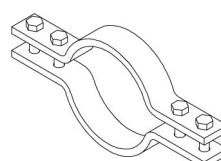
FIG. 590 FOUR BOLT UNDERGROUND PIPE CLAMP PAGE 77
