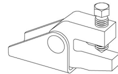
FIG. 030 C-CLAMP STRUCTURAL ATTACHMENT PAGE 118
